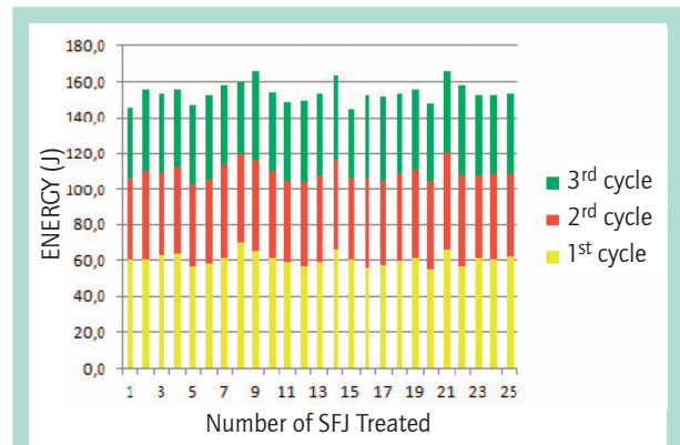
FIGURE 4 : 50 SFJ Energy developed by 2 Cycles
